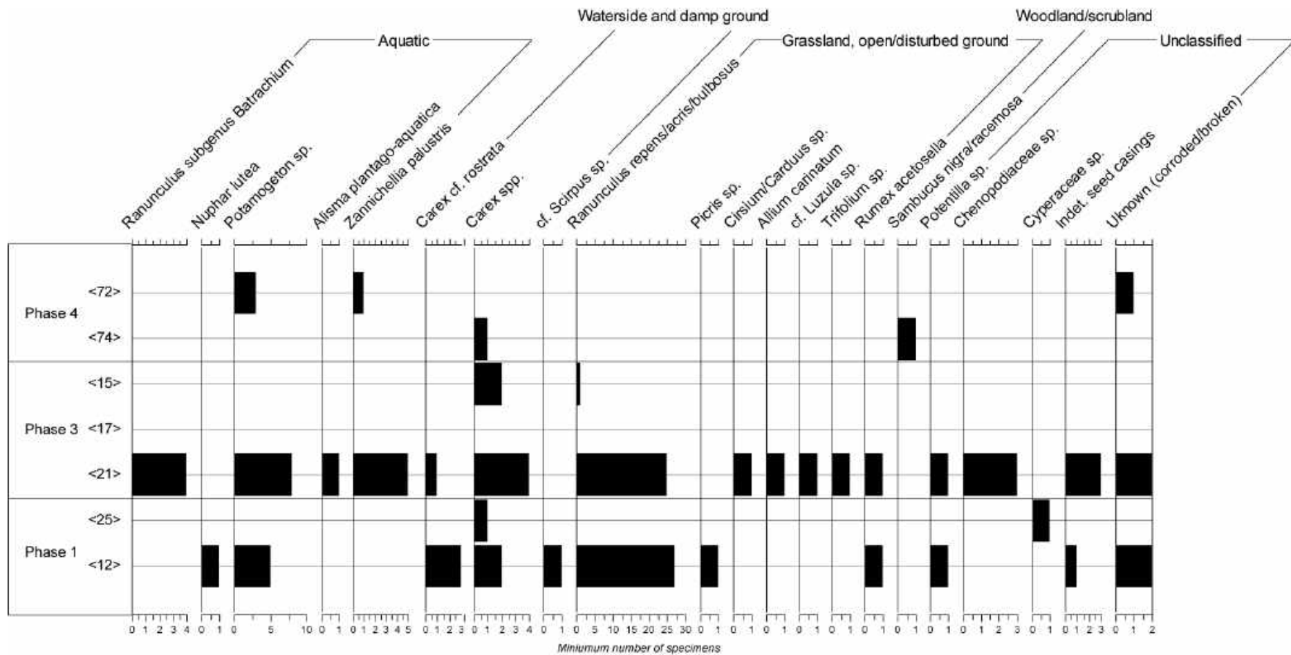
Figure 16. Results of the plant macrofossil analysis,
